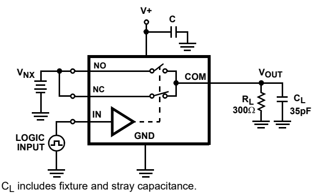
FIGURE 2D. TEST CIRCUIT (ISL84544 ONLY)
