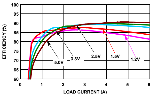
FIGURE 7. EFFICIENCY vs LOAD CURRENT ( 18\text{V}_{IN} )
