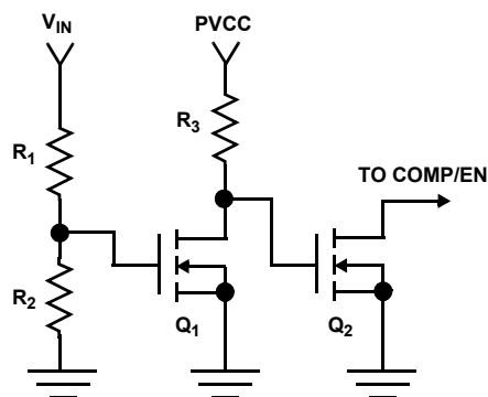
FIGURE 24. SEQUENCE CIRCUIT
