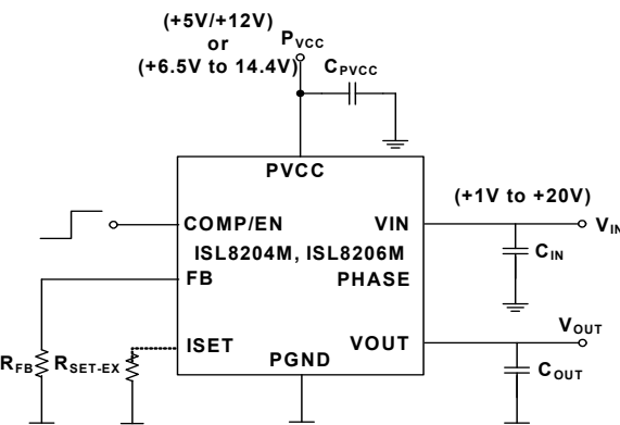
FIGURE 16. WIDE INPUT VOLTAGE APPLICATION SCHEMATIC
