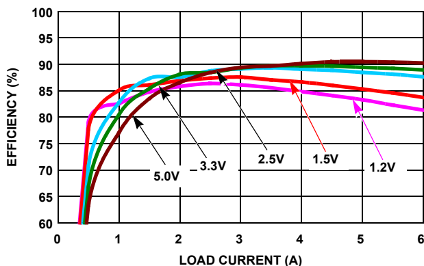
FIGURE 7. EFFICIENCY vs LOAD CURRENT ( 18V_{IN} )
