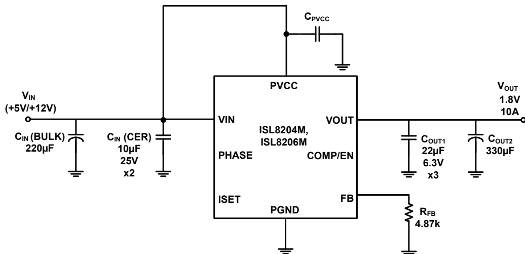
FIGURE 4. TEST CIRCUIT FOR ALL PERFORMANCE AND DERATING GRAPHS
