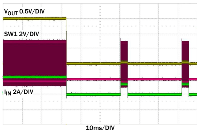
FIGURE 19. OUTPUT SHORT-CIRCUIT PROTECTION, HICCUP MODE
