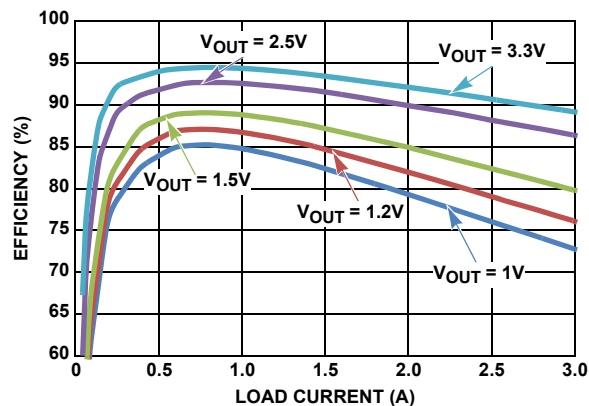
FIGURE 5. SINGLE CHANNEL, EN1 = HIGH, EN2 = LOW, V_{IN} = 5\text{V}
