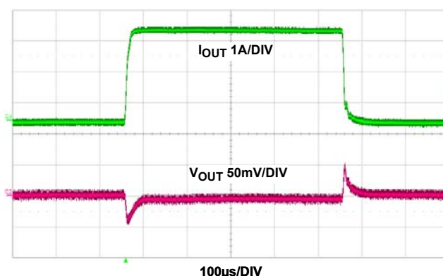
FIGURE 17. V_{IN} = 5V , V_{OUT} = 3.3V , I_{OUT} = 0 TO 3A , f_{SW} = 2MHz , C_{OUT} = 2 \times 22\mu F CERAMIC CAPACITORS
