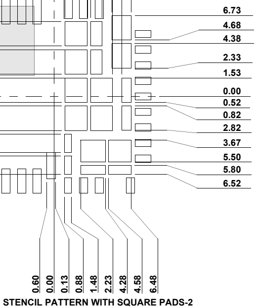
STENCIL PATTERN WITH SQUARE PADS-2
