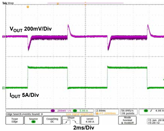
Figure 22. Load Transient, V_{IN} = 12V , I_{OUT} = 0A to 10A , 2.5A/\mu s , CCM
