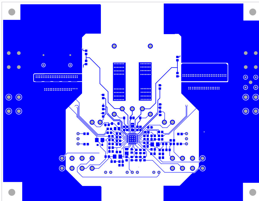
Figure 9. Top Layer
