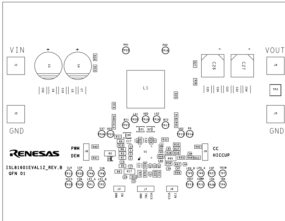
Figure 8. Silkscreen Top
