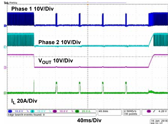
Figure 27. Short-Circuit Waveform
