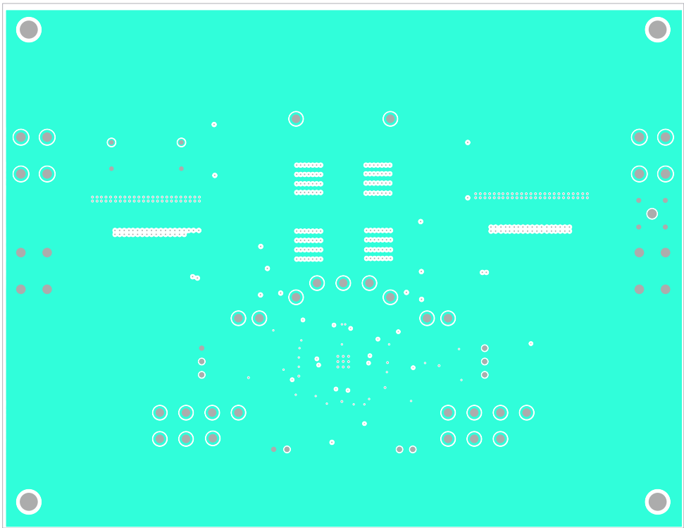
Figure 10. Third Layer
