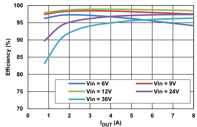
Figure 14. Efficiency, DEM
