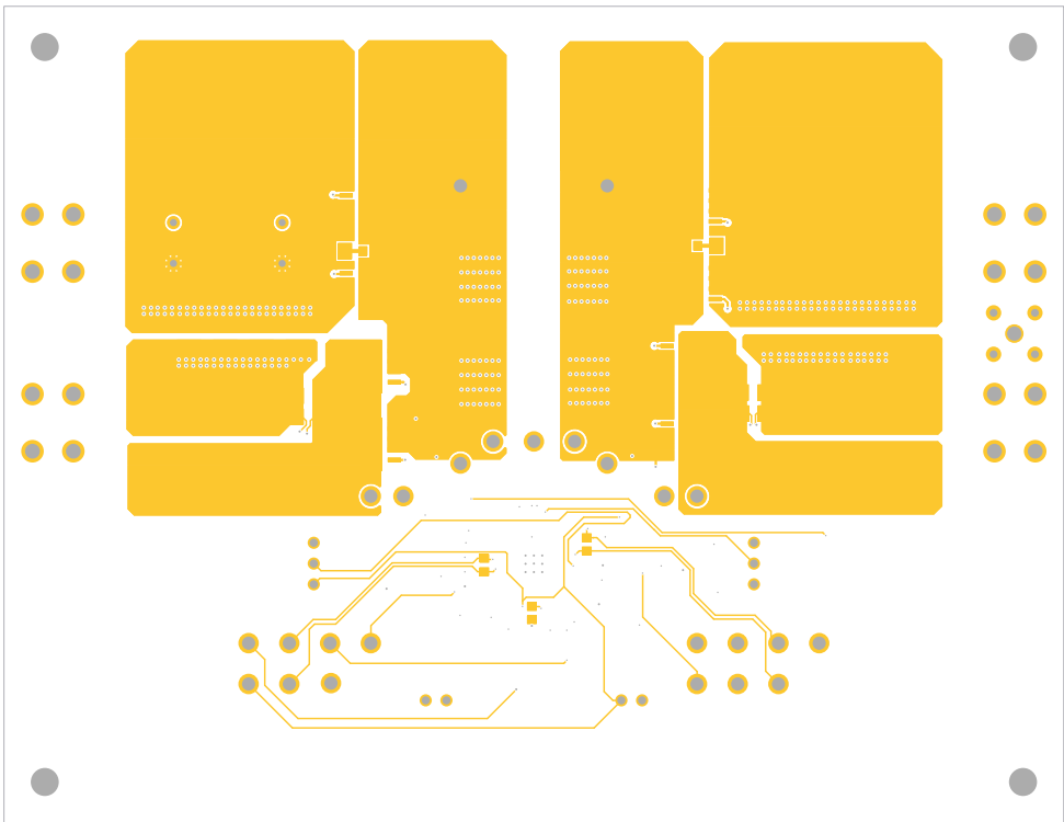
Figure 11. Bottom Layer
