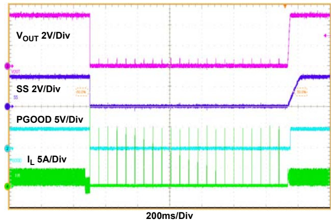
Figure 19. Short-Circuit Waveforms
