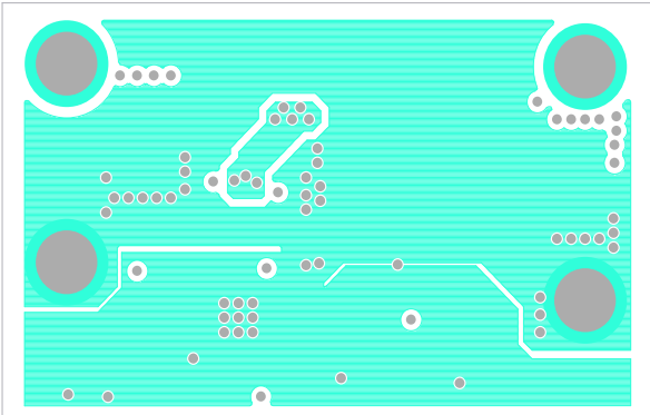
Figure 10. Third Layer
