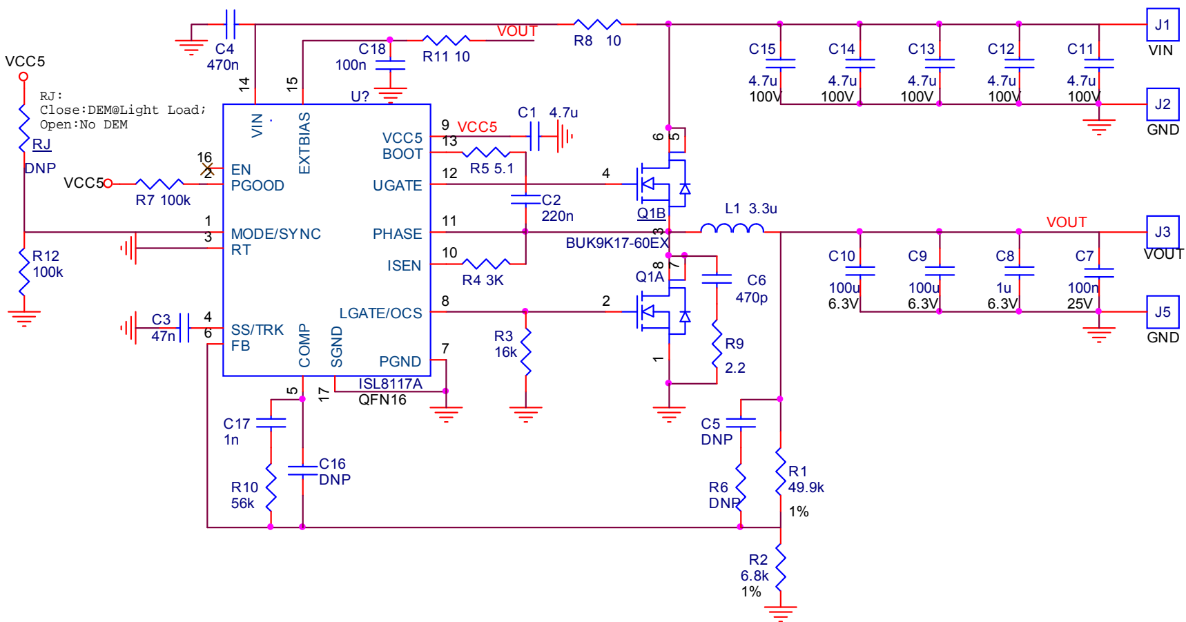
Figure 6. ISL8117ADEMO3Z Schematic
