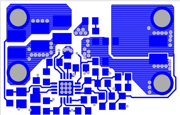
Figure 8. Top Layer
