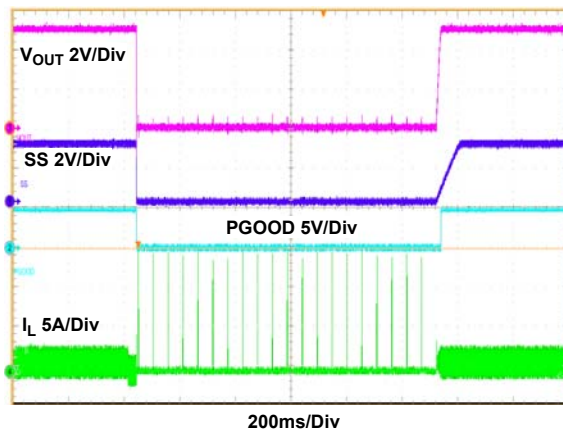
Figure 19. Short-Circuit Waveforms
