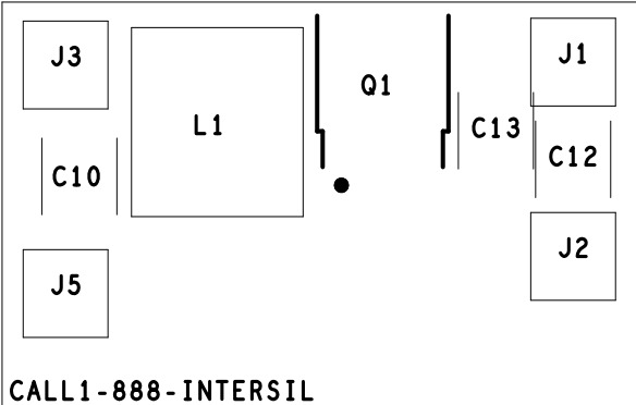
Figure 12. Assembly Bottom
