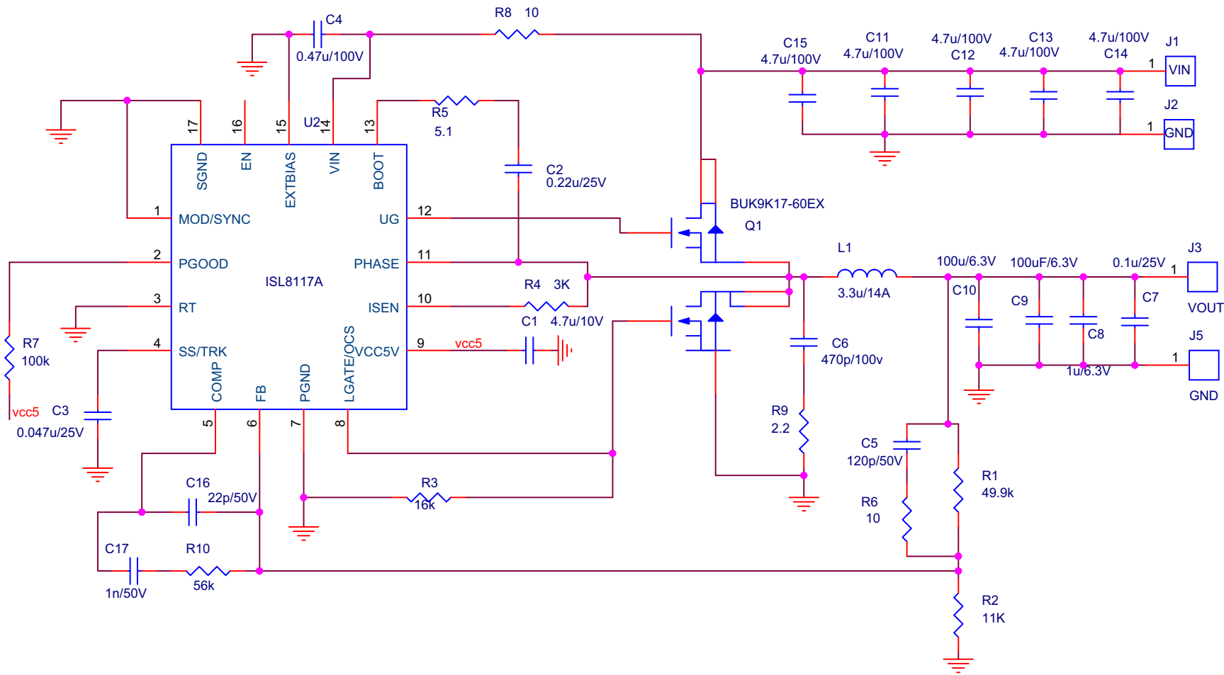
FIGURE 6. ISL8117ADEMO1Z SCHEMATIC
