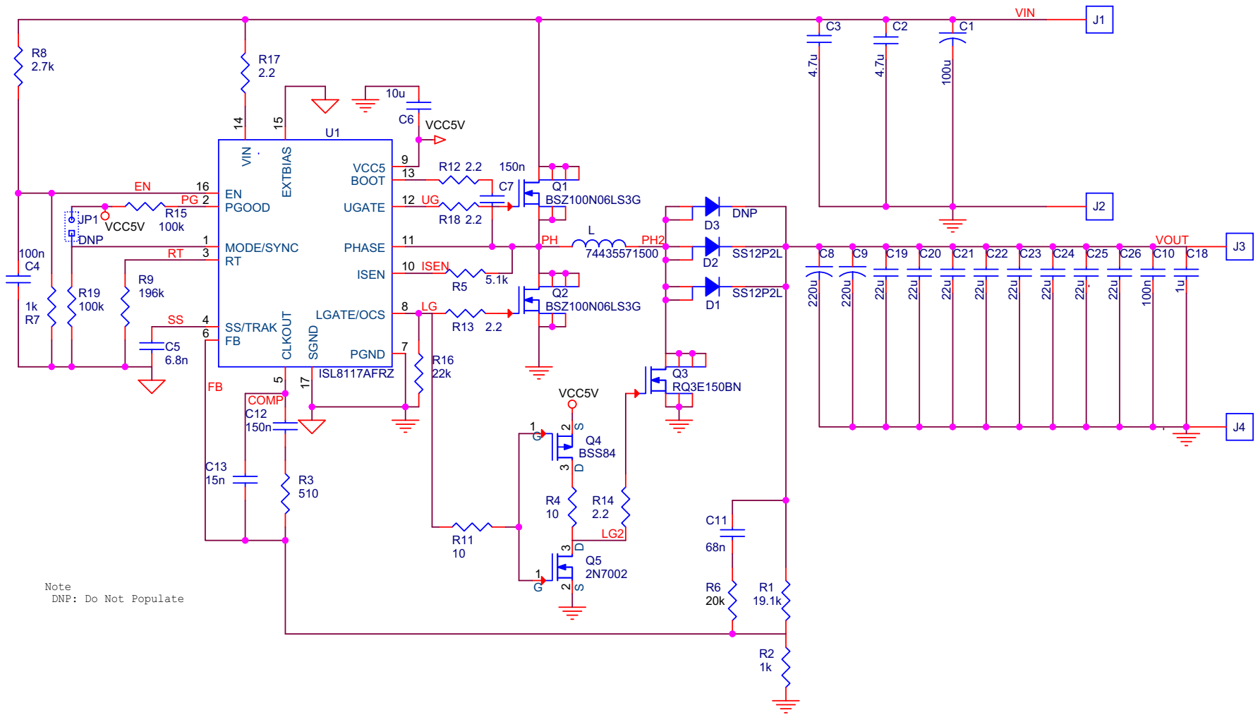
FIGURE 6. ISL8117A-LDEMO2Z SCHEMATIC
