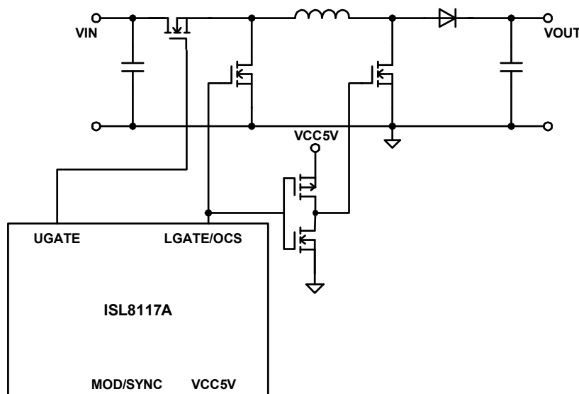
FIGURE 1. BLOCK DIAGRAM
