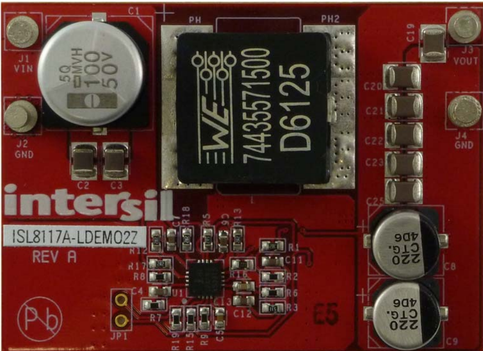
FIGURE 4. TOP VIEW
