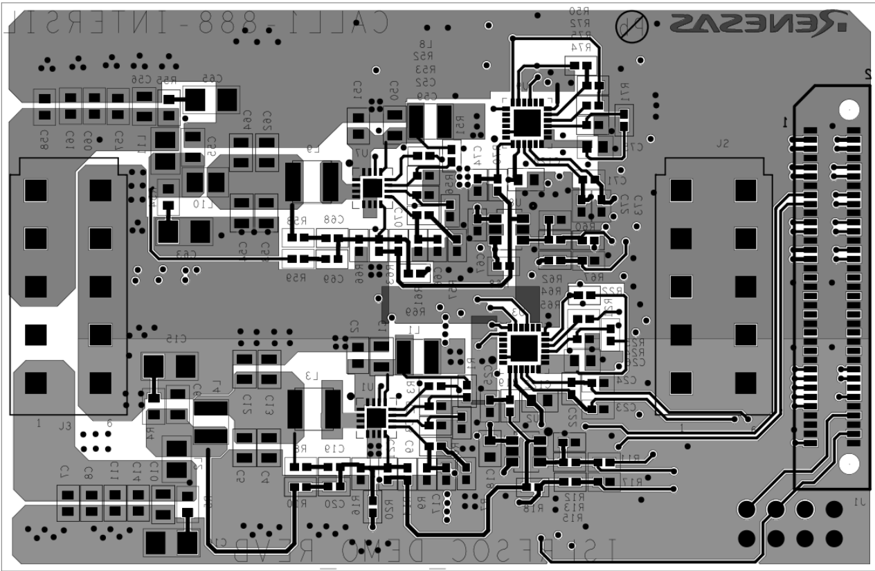
Figure 11. Bottom Layer
