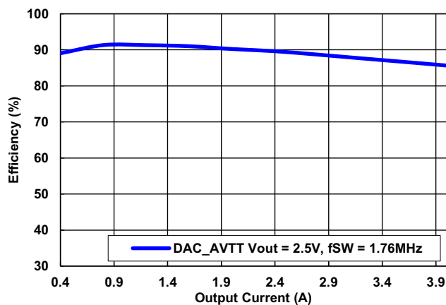
Figure 16. 5.DAC_AVTT Rail, Peak Efficiency = 92%
