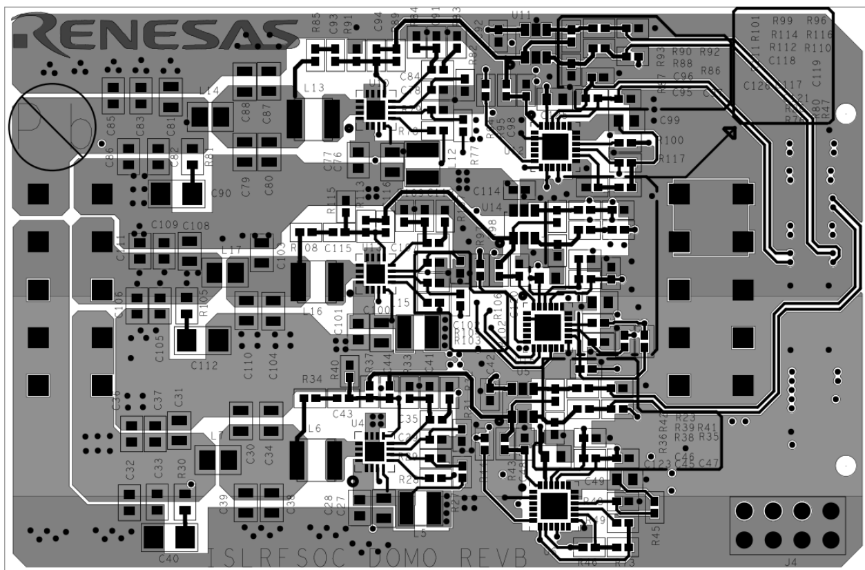
Figure 10. Top Layer
