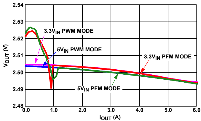
FIGURE 15. V_{OUT} REGULATION vs LOAD (1MHz, V_{OUT} = 2.5\text{V} )
