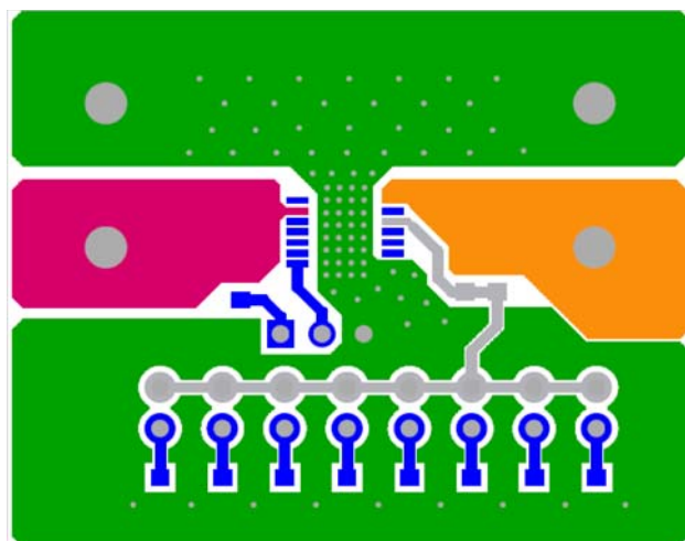
FIGURE 9. ISL80138EVAL1Z TOP
