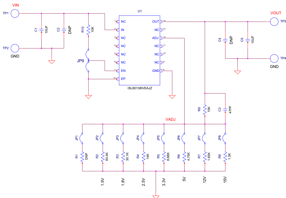
FIGURE 4. ISL80138EVAL1Z SCHEMATIC
