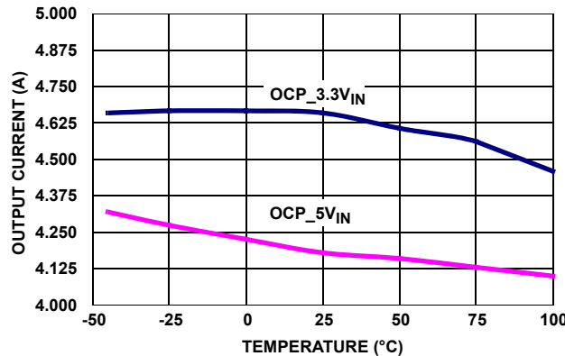
FIGURE 34. OUTPUT CURRENT LIMIT vs TEMPERATURE
