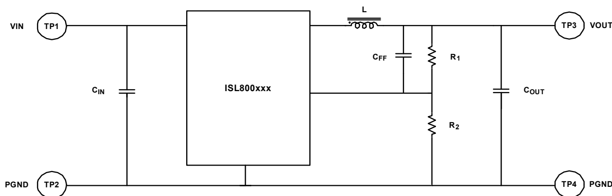
FIGURE 1. BLOCK DIAGRAM
