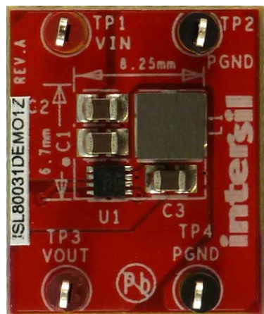
FIGURE 4. ISL80031DEMO1Z TOP SIDE
