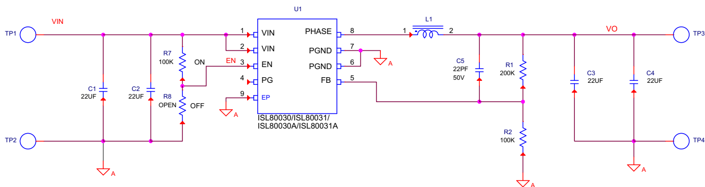
FIGURE 10. ISL8003xDEMO1Z SCHEMATIC
