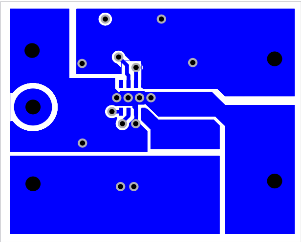
FIGURE 4. LAYER 1
