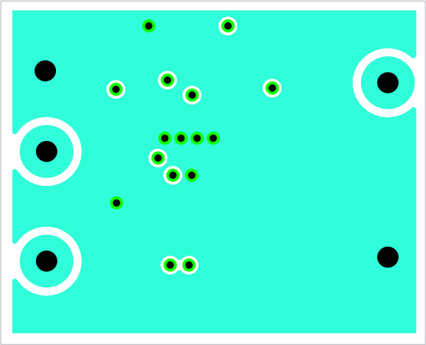
FIGURE 6. LAYER 3
