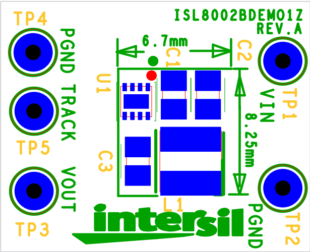
FIGURE 3. SILKSCREEN TOP
