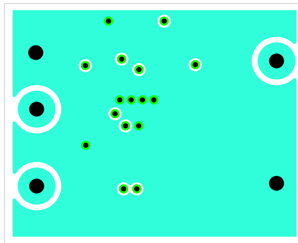
FIGURE 6. LAYER 3
