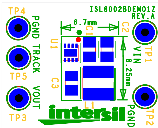
FIGURE 3. SILKSCREEN TOP
