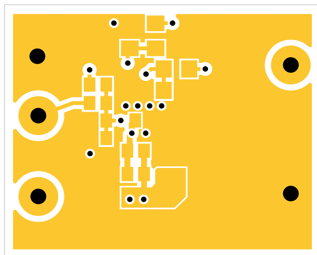
FIGURE 7. LAYER 4
