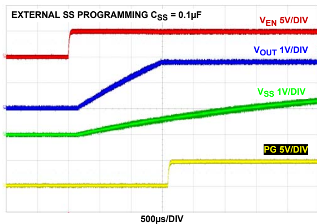
FIGURE 9. START-UP AT 2A LOAD f_{SW} = 2MHz , V_{IN} = 5V , MODE = PWM, T_A = +25^\circ C
