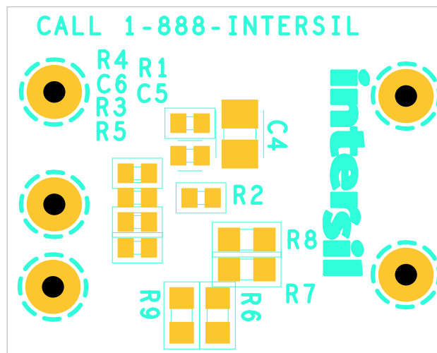
FIGURE 8. SILKSCREEN BOTTOM
