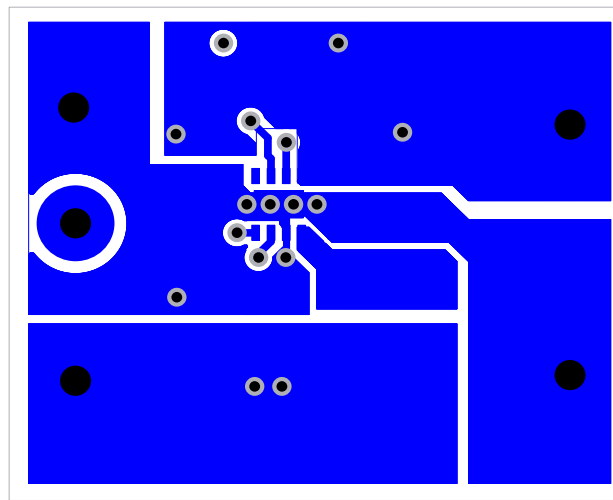
FIGURE 4. LAYER 1
