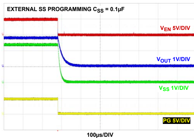
FIGURE 10. SHUTDOWN AT 2A LOAD f_{SW} = 2MHz , V_{IN} = 5V , MODE = PWM, T_A = +25^\circ C
