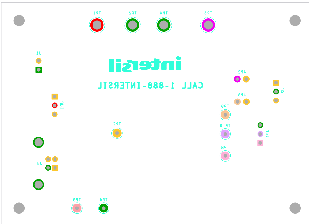
FIGURE 10. SILKSCREEN BOTTOM
