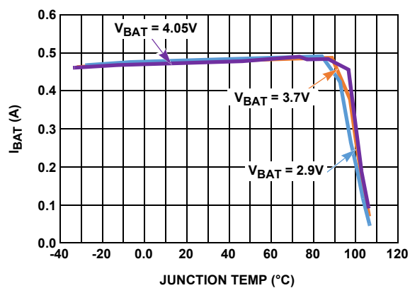
FIGURE 16. CHARGE CURRENT vs JUNCTION TEMPERATURE, R_{IREF} = 158k
