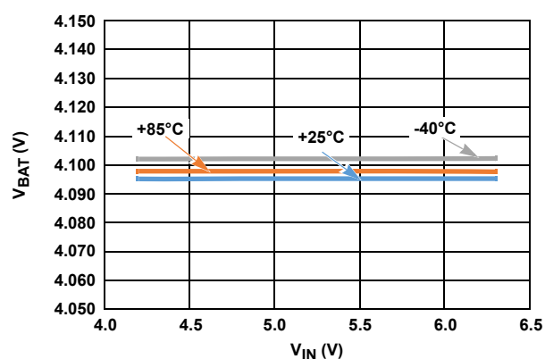
FIGURE 13. NO LOAD VOLTAGE vs TEMPERATURE
