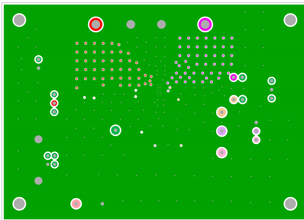
FIGURE 7. INTERNAL (LAYER 2)
