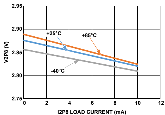
FIGURE 19. V2P8 OUTPUT vs LOAD CURRENT
