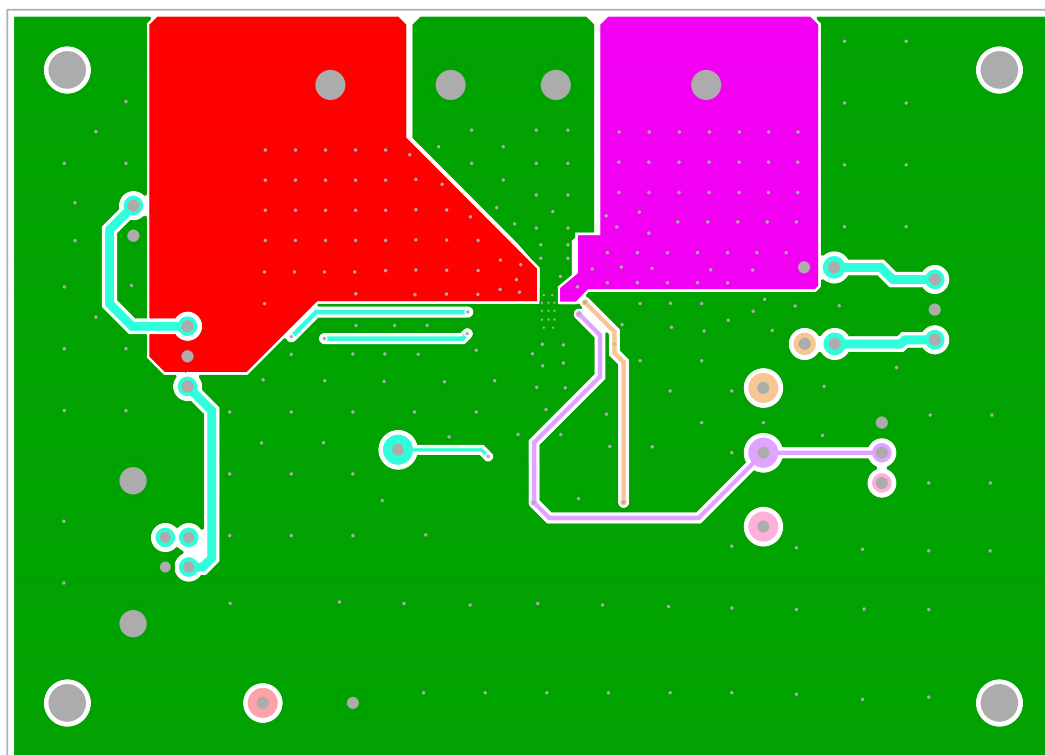
FIGURE 8. INTERNAL (LAYER 3)
