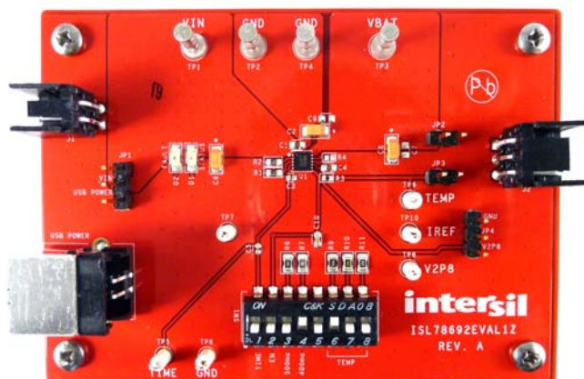
FIGURE 1. TOP VIEW
