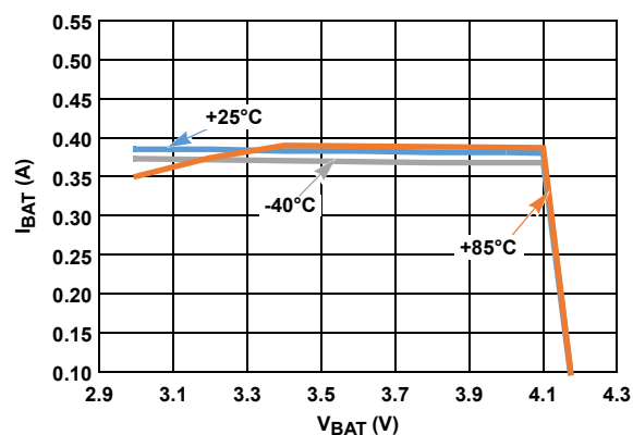
FIGURE 15. CHARGE CURRENT vs OUTPUT VOLTAGE, R_{IREF} = 200k
