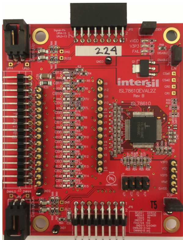
FIGURE 11. TOP VIEW
