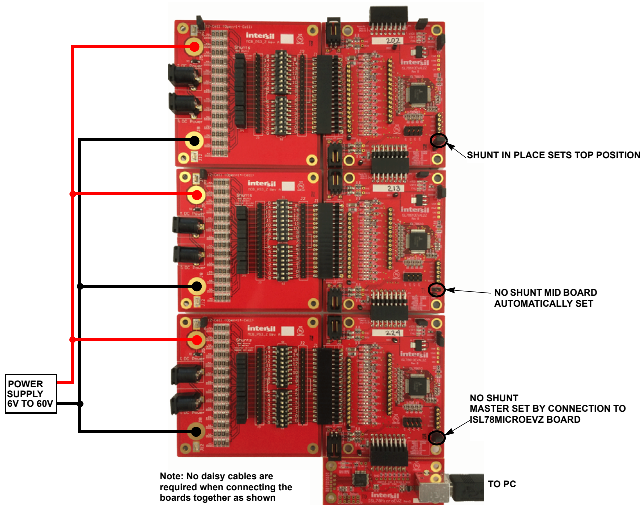
FIGURE 3. ISL78610EVKIT1Z IN 36-CELL DAISY CHAIN CONFIGURATION
