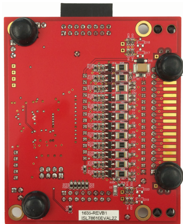
FIGURE 12. BOTTOM VIEW
