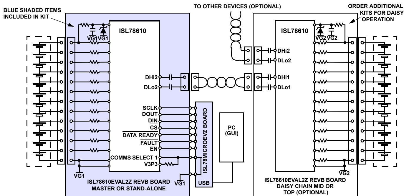
FIGURE 1. TYPICAL APPLICATION
