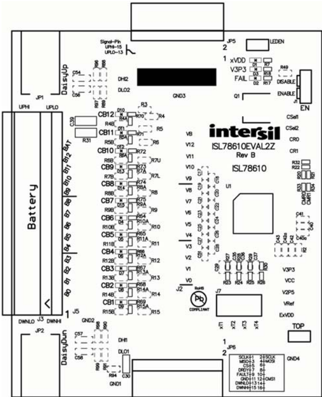
FIGURE 19. ISL78610EVAL2Z REVB TOP OVERLAY
