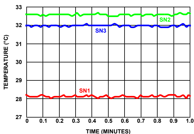
FIGURE 28. INTERNAL TEMPERATURE DEVICE TO DEVICE SPREAD 48V
