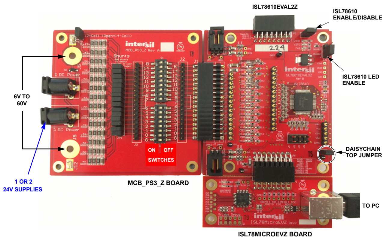
FIGURE 2. ISL78610EVKIT1Z REV B SINGLE BOARD SETUP
