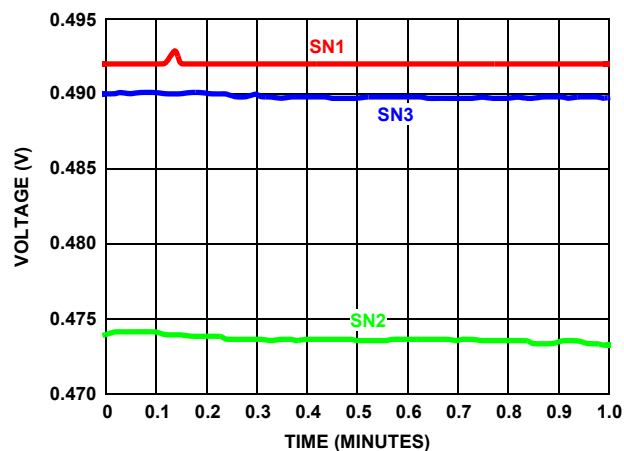
FIGURE 26. ETV1 DEVICE TO DEVICE SPREAD 48V
