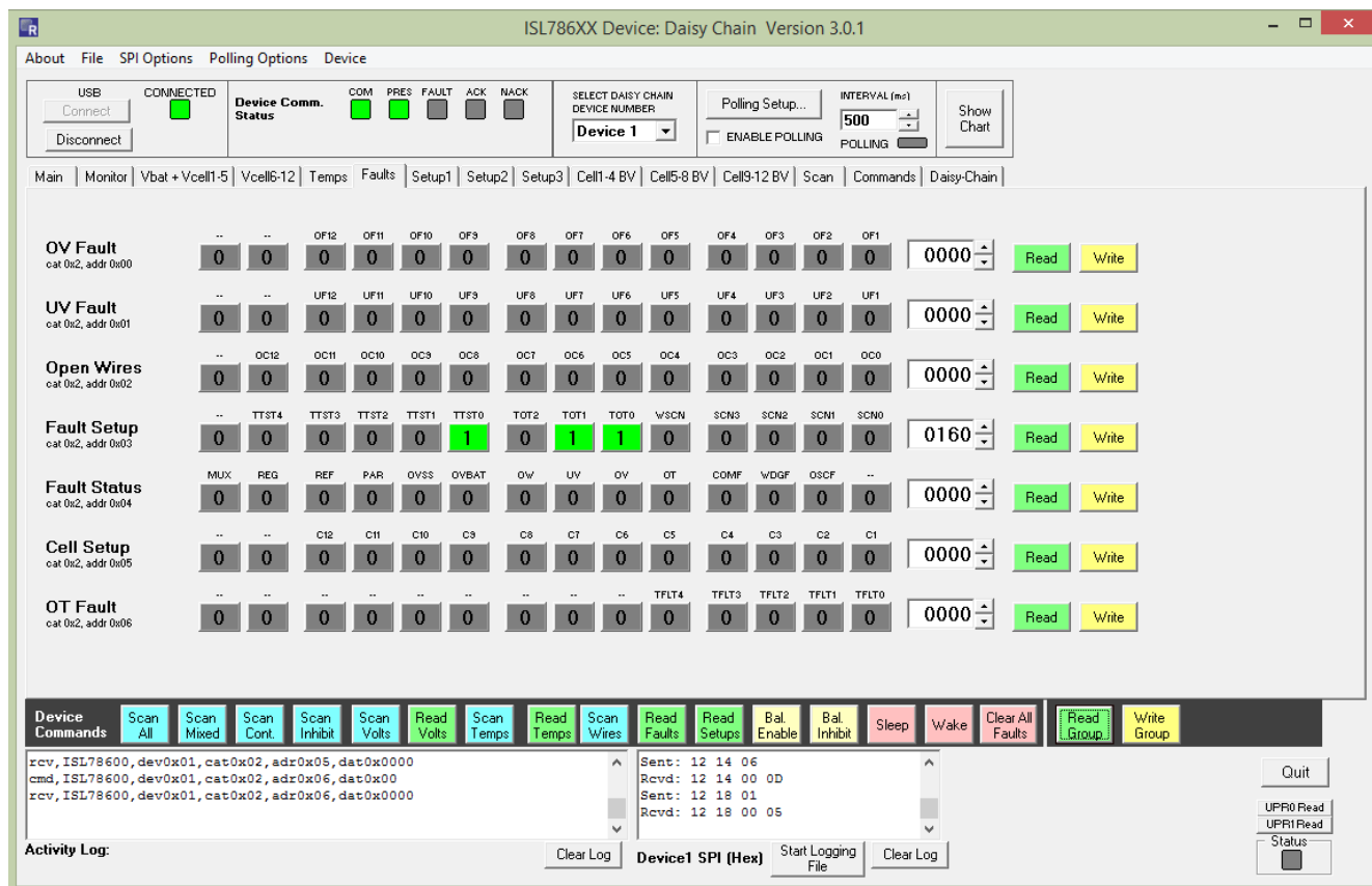
Figure 14. Fault Registers
