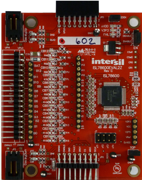
Figure 16. Top View
