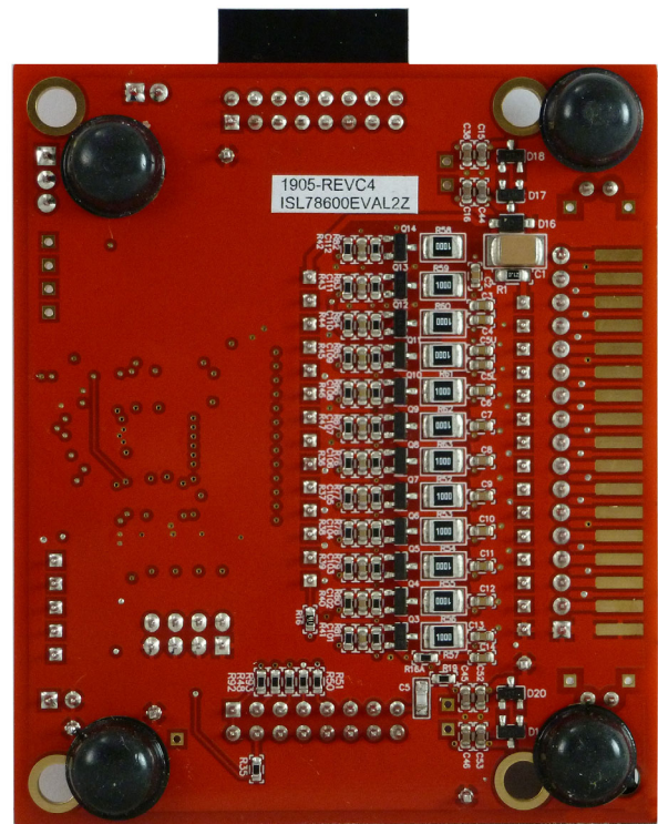
Figure 17. Bottom View
