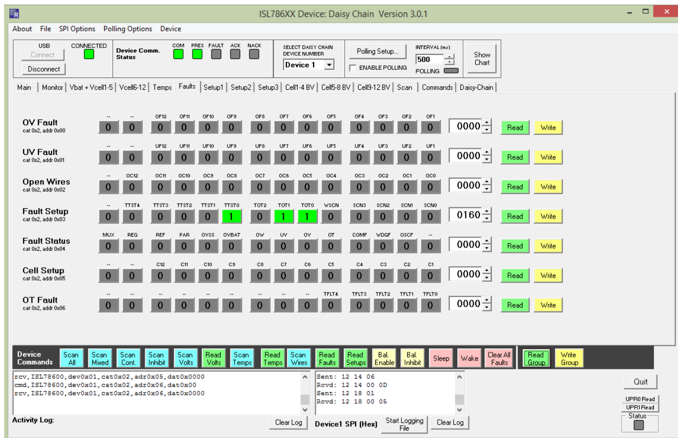
Figure 14. Fault Registers
