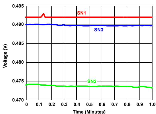
Figure 33. ETV1 Device to Device Spread 48V
