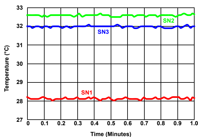
Figure 35. Internal Temperature Device to Device Spread 48V
