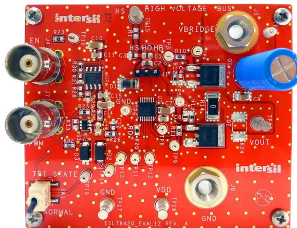
FIGURE 1. ISL78420EVAL1Z EVALUATION BOARD
