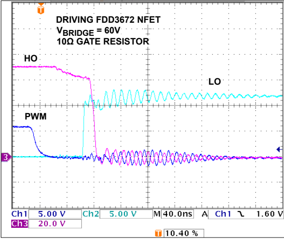
FIGURE 13. PWM, LO AND HO PULSE WAVEFORM
