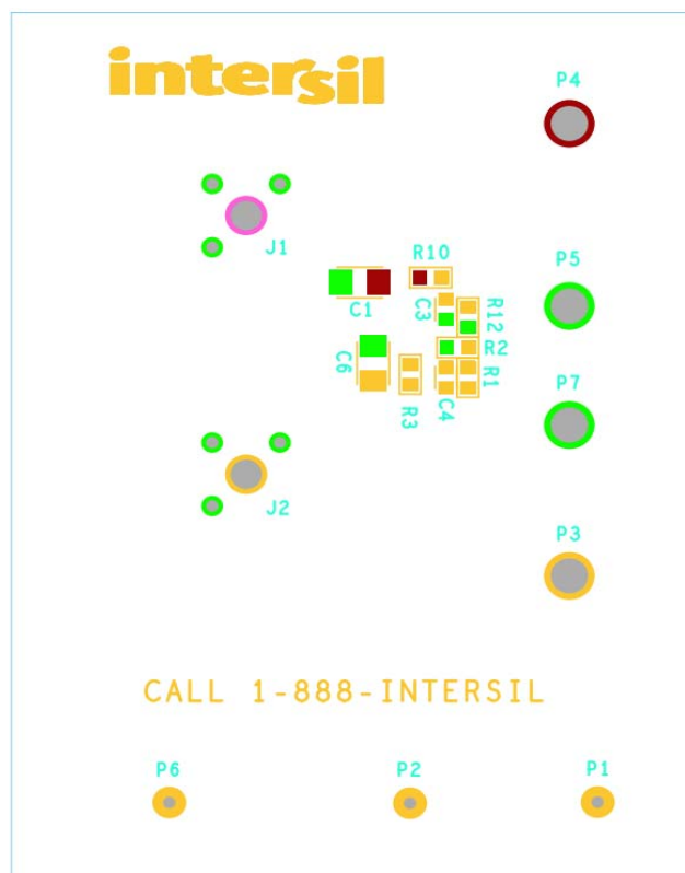
FIGURE 4. BOTTOM LAYER SILKSCREEN
