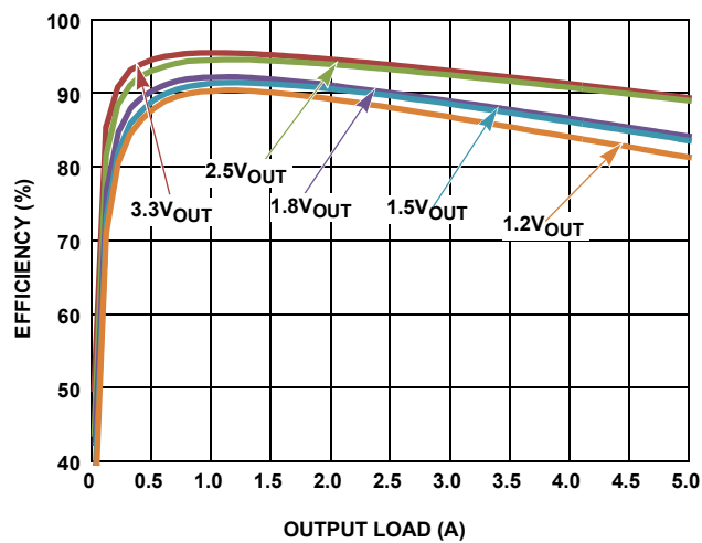
FIGURE 7. EFFICIENCY vs LOAD ( 5\text{V}_{IN} ; \text{SYNC} = V_{DD} )
