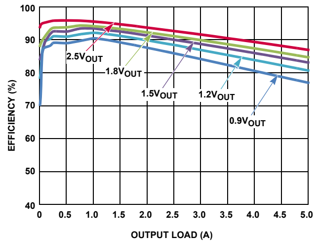
FIGURE 6. EFFICIENCY vs LOAD ( 3.3\text{V}_{IN} ; \text{SYNC} = \text{GND} )
