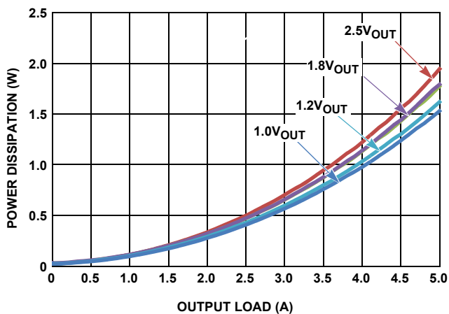
FIGURE 9. POWER DISSIPATION vs LOAD ( 3.3\text{V}_{IN} ; \text{SYNC} = V_{DD} )
