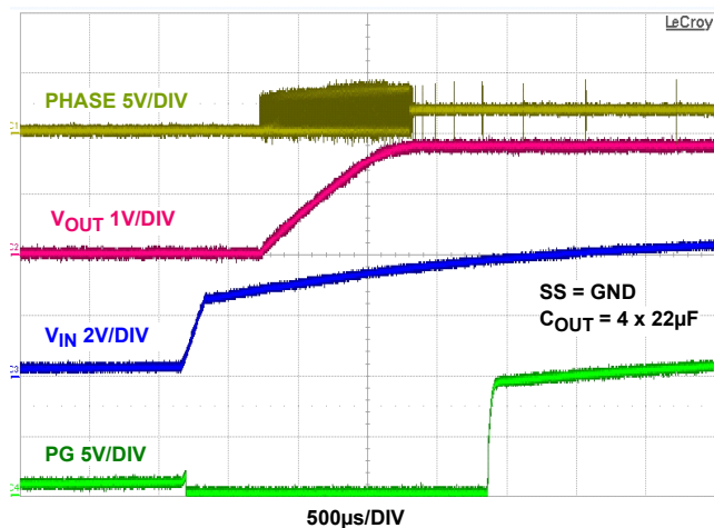
FIGURE 17. V_{IN} START-UP AT NO LOAD ( \text{SYNC} = \text{GND} )
