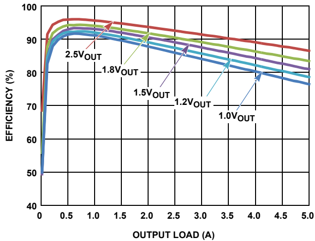
FIGURE 5. EFFICIENCY vs LOAD ( 3.3\text{V}_{IN} ; \text{SYNC} = V_{DD} )
