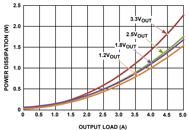
FIGURE 10. POWER DISSIPATION vs LOAD ( 5\text{V}_{IN} ; \text{SYNC} = V_{DD} )
