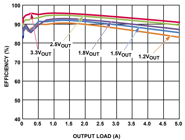
FIGURE 8. EFFICIENCY vs LOAD ( 5\text{V}_{IN} ; \text{SYNC} = \text{GND} )
