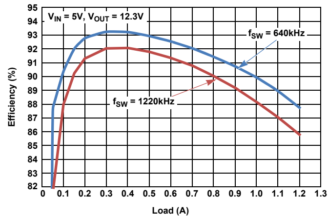
Figure 9. V_{OUT} = 12.3V Efficiency
