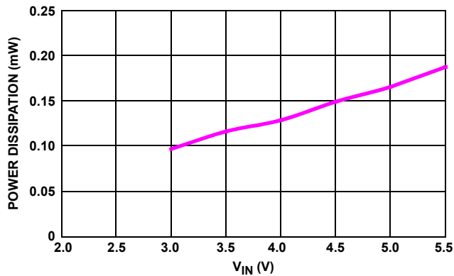
FIGURE 9. POWER DISSIPATION WITH NO LOAD vs V_{\text{IN}} (PFM V_{\text{OUT}} = 1.8\text{V} )
