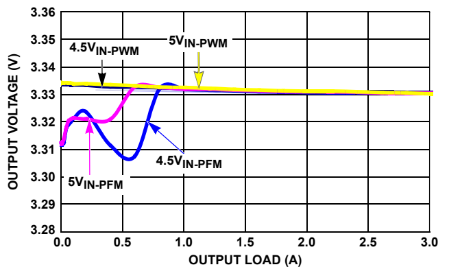
FIGURE 14. V_{\text{OUT}} REGULATION vs LOAD (1MHz, V_{\text{OUT}} = 3.3\text{V} )
