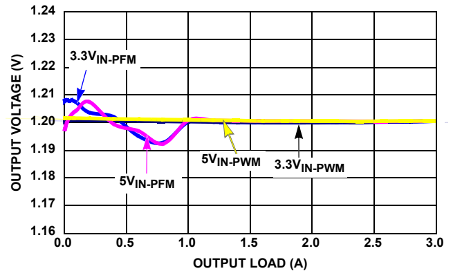
FIGURE 10. V_{\text{OUT}} REGULATION vs LOAD (1MHz, V_{\text{OUT}} = 1.2\text{V} )
