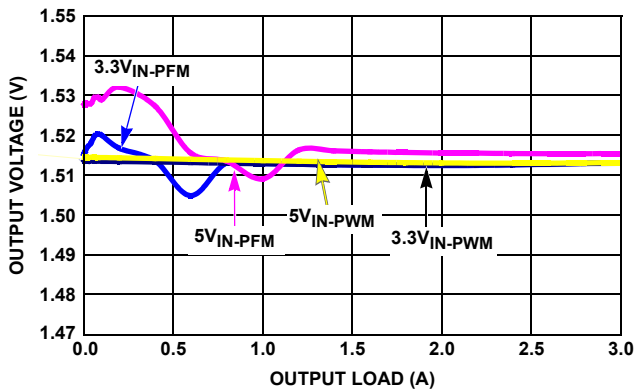
FIGURE 11. V_{\text{OUT}} REGULATION vs LOAD (1MHz, V_{\text{OUT}} = 1.5\text{V} )
