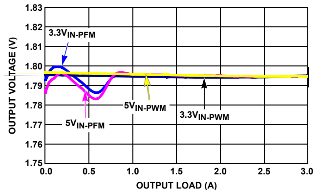
FIGURE 12. V_{\text{OUT}} REGULATION vs LOAD (1MHz, V_{\text{OUT}} = 1.8\text{V} )
