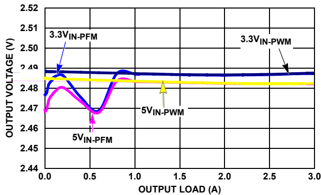
FIGURE 13. V_{\text{OUT}} REGULATION vs LOAD (1MHz, V_{\text{OUT}} = 2.5\text{V} )
