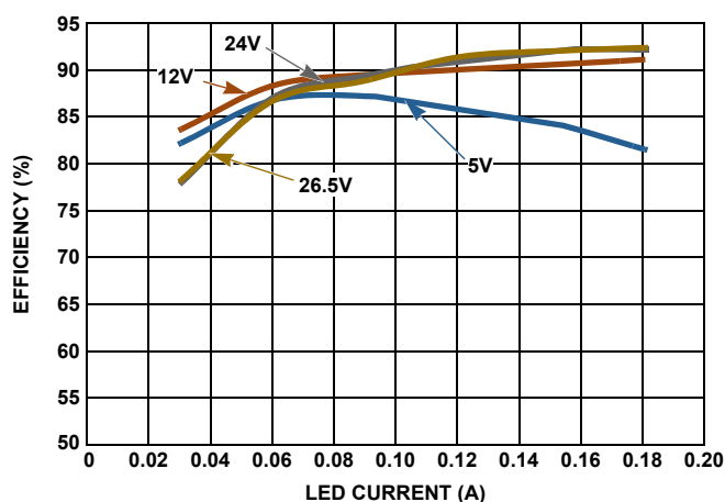
FIGURE 10. EFFICIENCY vs LED CURRENT AT LX FREQUENCY = 600kHz AT 25^{\circ}\text{C} vs V_{\text{IN}}
