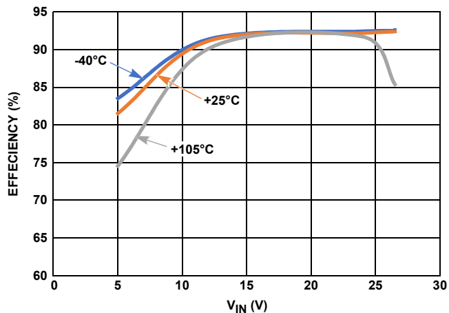
FIGURE 12. EFFICIENCY vs INPUT VOLTAGE AT LX FREQUENCY = 600kHz vs V_{\text{IN}}
