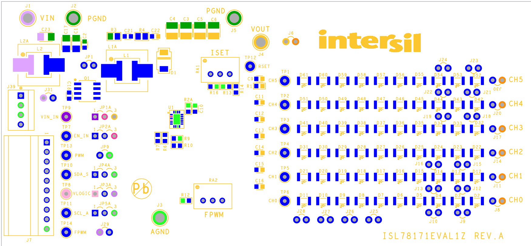
FIGURE 3. SILKSCREEN TOP
