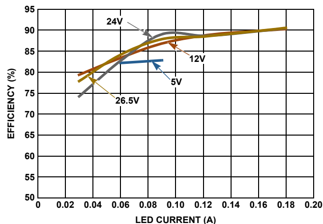
FIGURE 14. EFFICIENCY vs LED CURRENT AT LX FREQUENCY = 1.2MHz AT 25^{\circ}\text{C} vs V_{\text{IN}}
