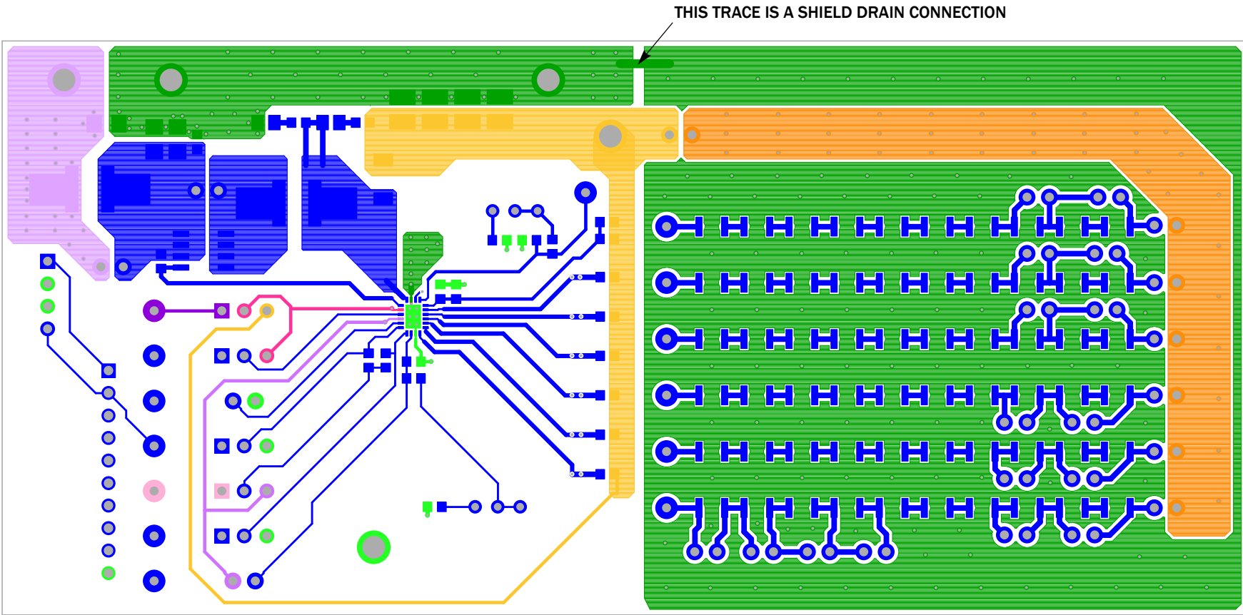
FIGURE 4. TOP LAYER
