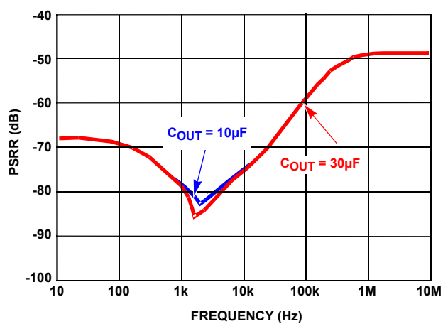
FIGURE 19. PSRR vs FREQUENCY ( V_{IN} = -7V , V_{OUT} = -5V )
