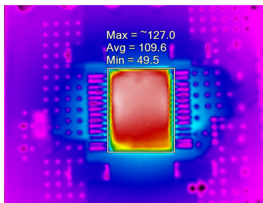
FIGURE 21. THERMAL ( V_{IN} = -12V , V_{OUT} = -5V , I_{OUT} = 0.74A , T_A = +25^{\circ}C )
