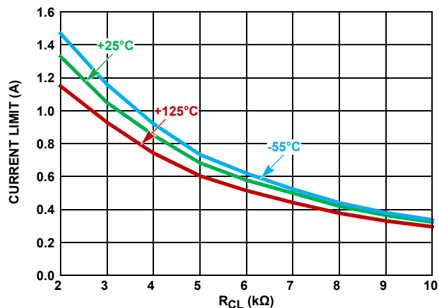
FIGURE 11. -12V_{IN} , -5V_{OUT}
