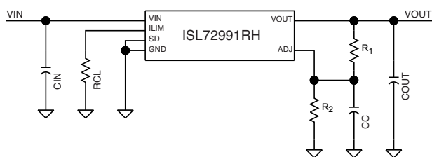
FIGURE 1. TYPICAL APPLICATION
