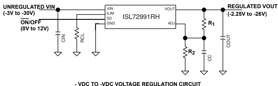
FIGURE 4. TYPICAL APPLICATION
