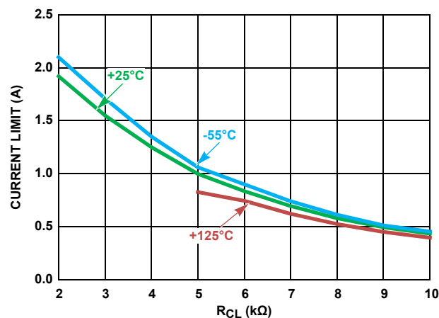
FIGURE 13. -20V_{IN} , -10V_{OUT}
