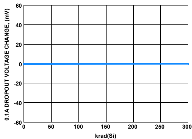
FIGURE 6. 0.1A DROPOUT VOLTAGE CHANGE vs TOTAL DOSE RADIATION
