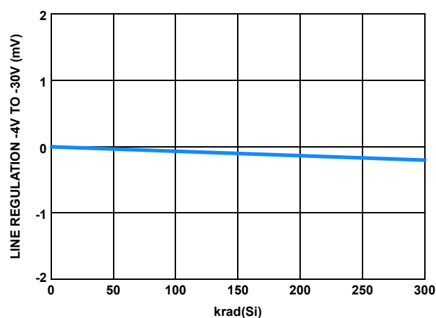
FIGURE 8. OUTPUT VOLTAGE LINE REGULATION CHANGE vs TOTAL DOSE RADIATION
