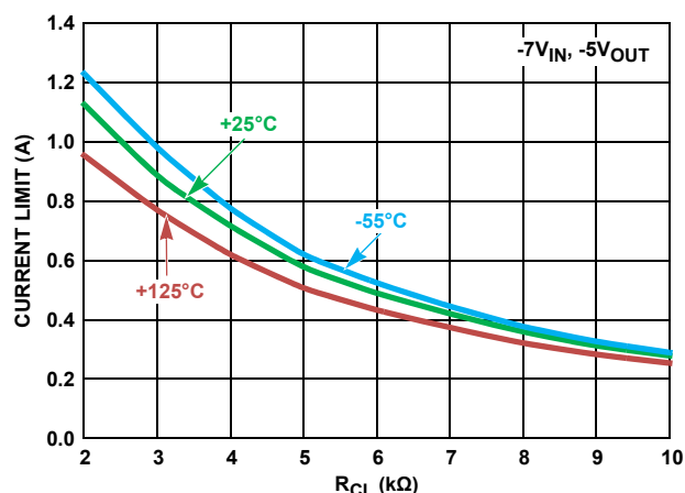
FIGURE 23. I_{CL} vs R_{CL} AND TEMPERATURE
