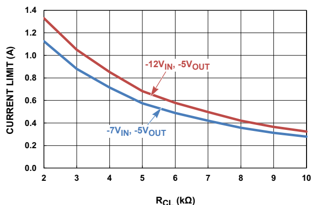
FIGURE 22. I_{CL} vs R_{CL} AND V_{IN} AMPLITUDE
