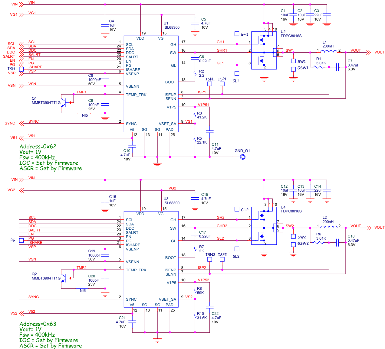
Figure 4. Schematic
