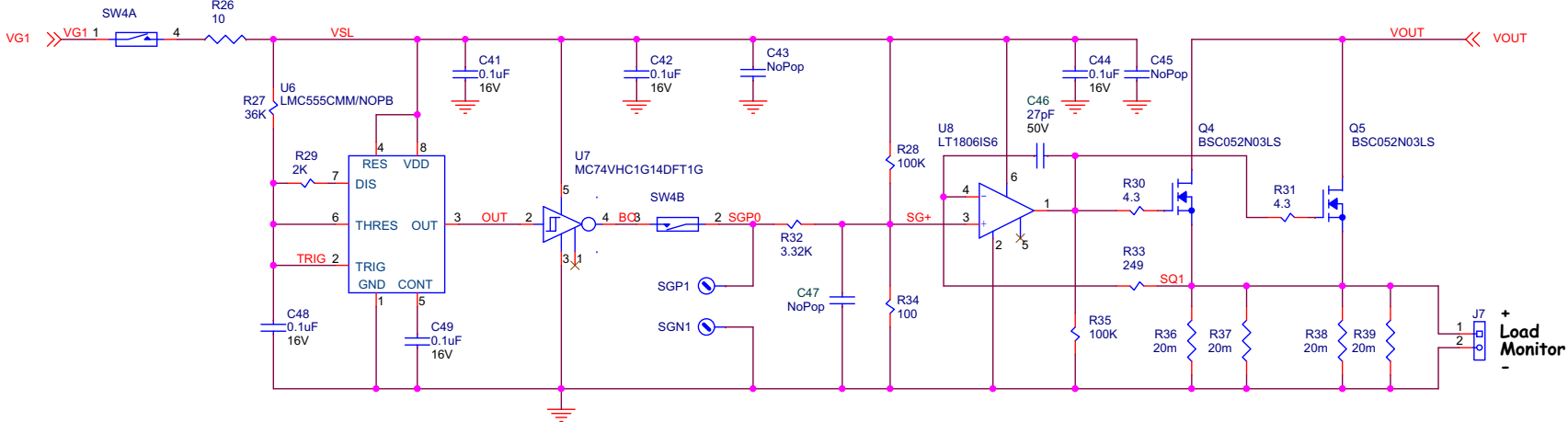
Figure 7. Schematic - Dynamic Load
