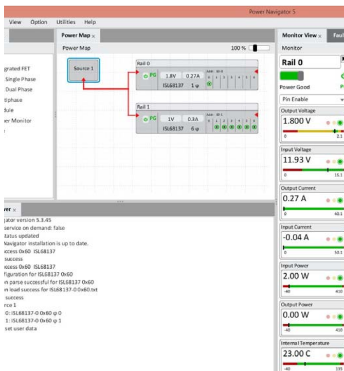
FIGURE 7. POWER MAP
