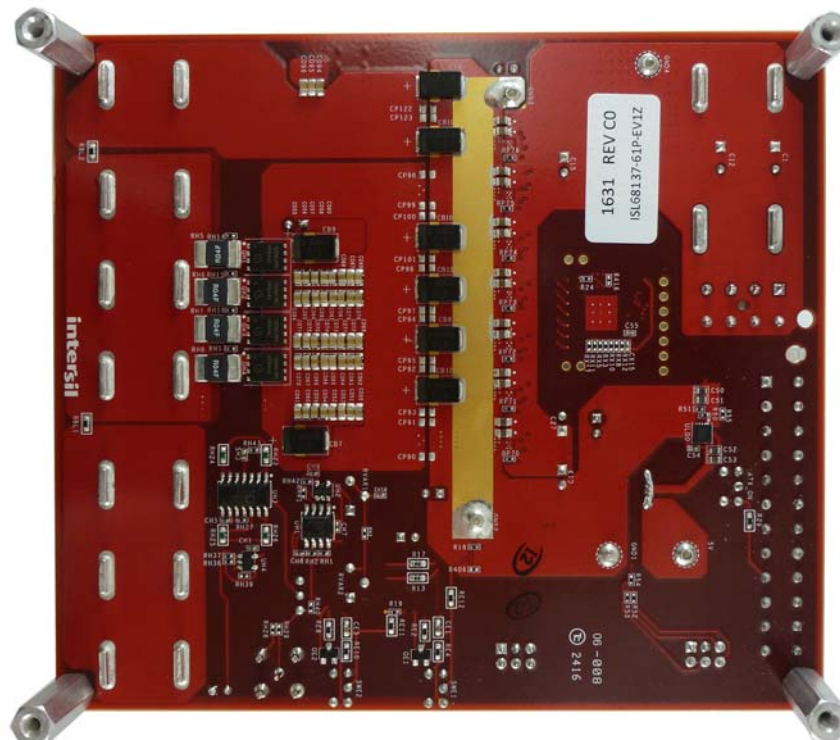
FIGURE 9. BOTTOM SIDE
