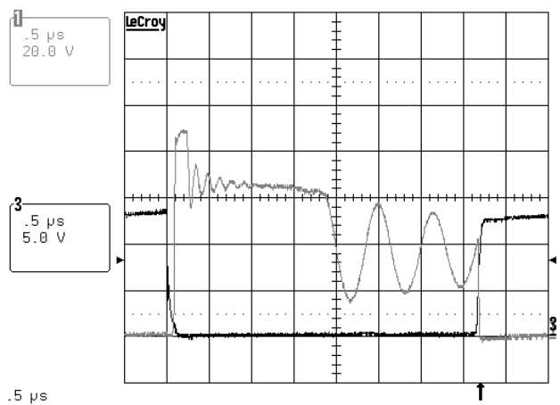
Figure 15 GATE AND DRAIN-SOURCE WAVEFORMS
