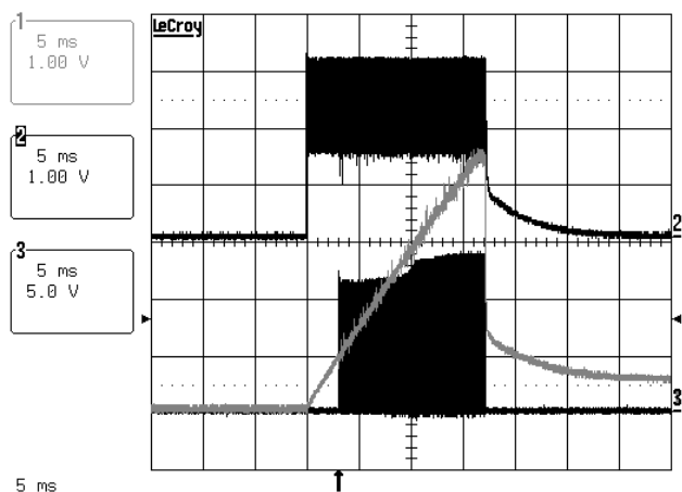
Figure 14 SOFT-START WITH OVERCURRENT FAULT
