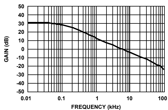
FIGURE 12A. GAIN
