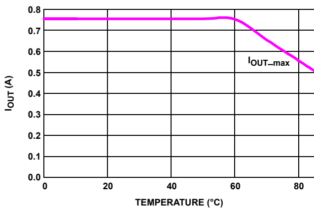
FIGURE 3. OUTPUT CURRENT DERATING (6x6 QFN)
