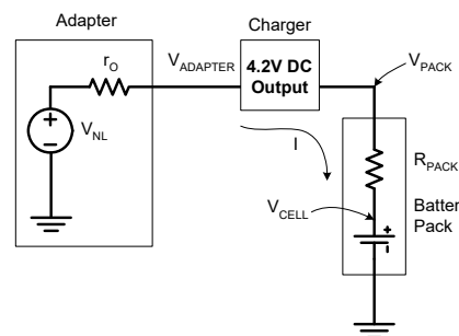
FIGURE 27C. THE EQUIVALENT CIRCUIT WHEN THE PACK VOLTAGE REACHES THE FINAL CHARGE VOLTAGE
