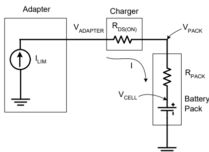
FIGURE 27A. THE EQUIVALENT CIRCUIT IN THE CONSTANT CURRENT REGION
