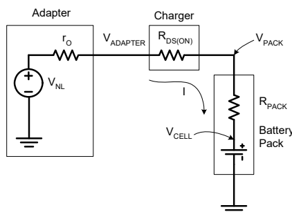
FIGURE 27B. THE EQUIVALENT CIRCUIT IN THE RESISTANCE-LIMIT REGION
