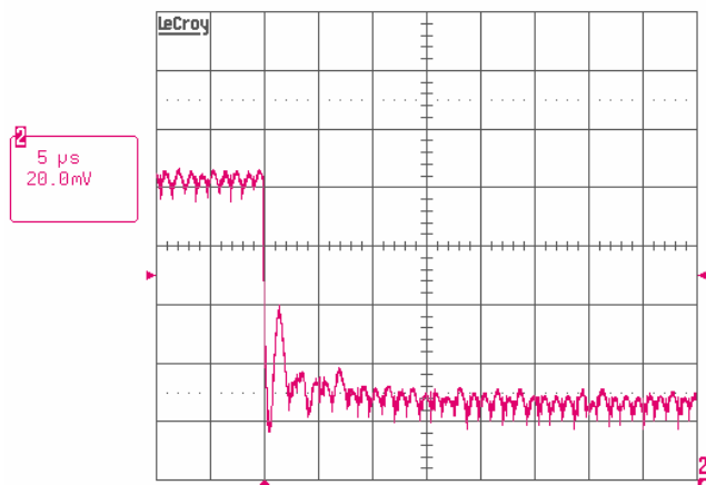
FIGURE 40. LOAD TRANSIENT RESPONSE WITH OVERSHOOT REDUCTION FUNCTION DISABLED, V_{IN} = 12V , SV CLARKSFIELD CPU TEST CONDITION: VID = 0.95V, I_O = 12A/51A , di/dt = "FASTEST", LL = 1.9mΩ
