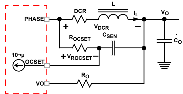
FIGURE 5. OVERCURRENT PROGRAMMING CIRCUIT
