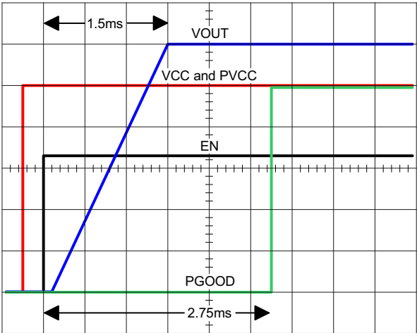
FIGURE 2. SOFT-START SEQUENCE
