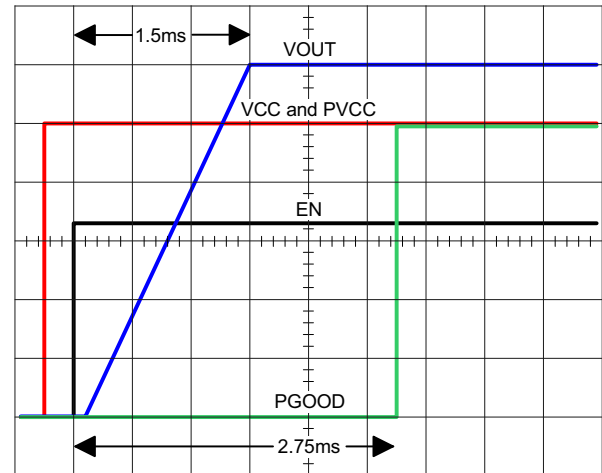
FIGURE 2. SOFT-START SEQUENCE
