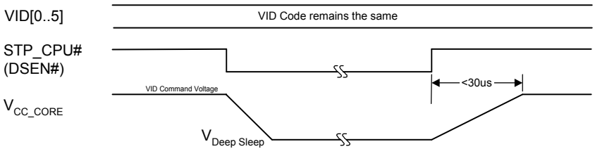
FIGURE 6. Vcore RESPONSE FOR DEEPER SLEEP COMMAND
