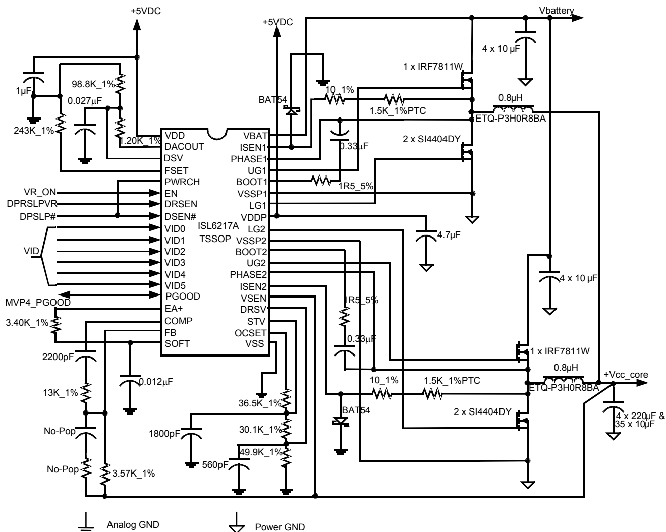
FIGURE 14. TYPICAL APPLICATION CIRCUIT FOR THE IMVP-IV™ AND IMVP-IV+™ CORE VOLTAGE REGULATOR
