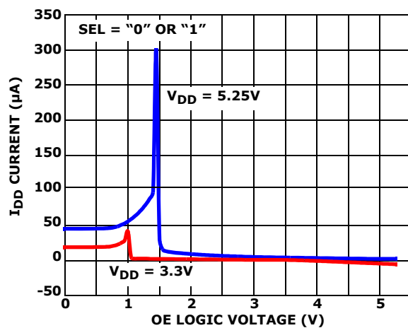
FIGURE 18. I_{DD} vs OE LOGIC VOLTAGE vs V_{DD}
