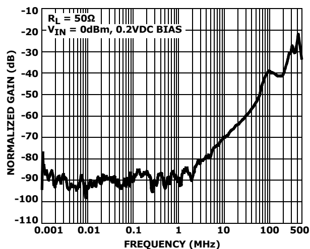
FIGURE 25. CROSSTALK
