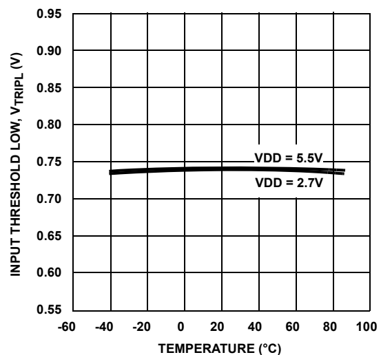
FIGURE 4. V_{TRIPL} VOLTAGE
