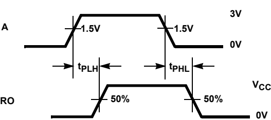
FIGURE 4B. MEASUREMENT POINTS
