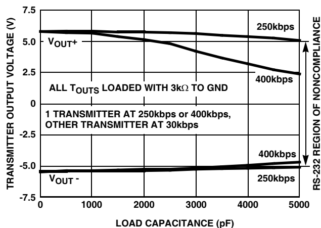
FIGURE 33. RS-232, TRANSMITTER OUTPUT VOLTAGE vs LOAD CAPACITANCE
