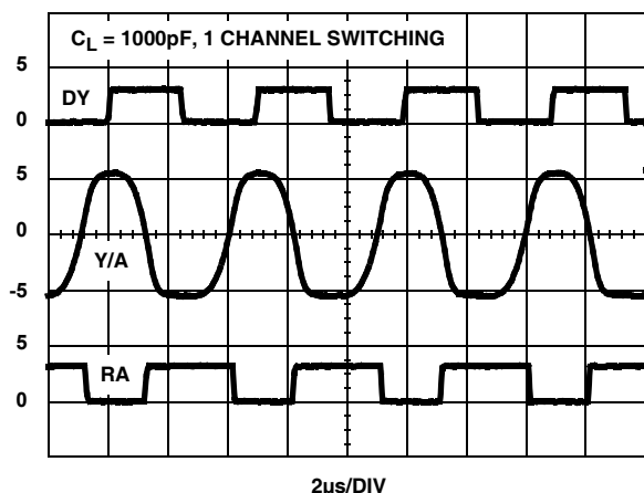
FIGURE 37. RS-232, TRANSMITTER AND RECEIVER WAVEFORMS AT 400kbps
