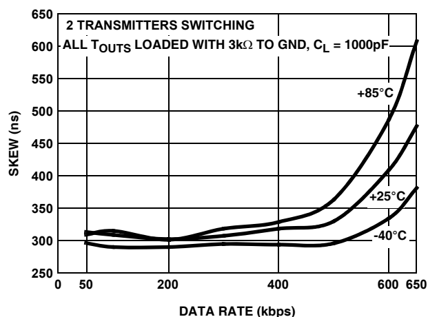
FIGURE 41. RS-232, TRANSMITTER SKEW vs DATA RATE
