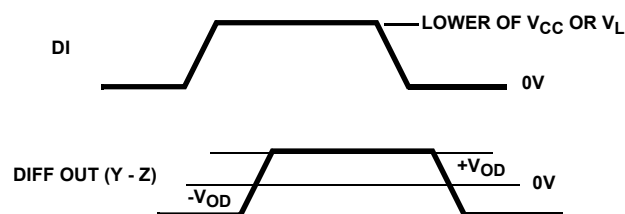
FIGURE 7B. MEASUREMENT POINTS
