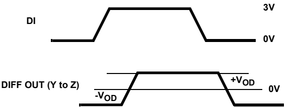
FIGURE 5B. MEASUREMENT POINTS
