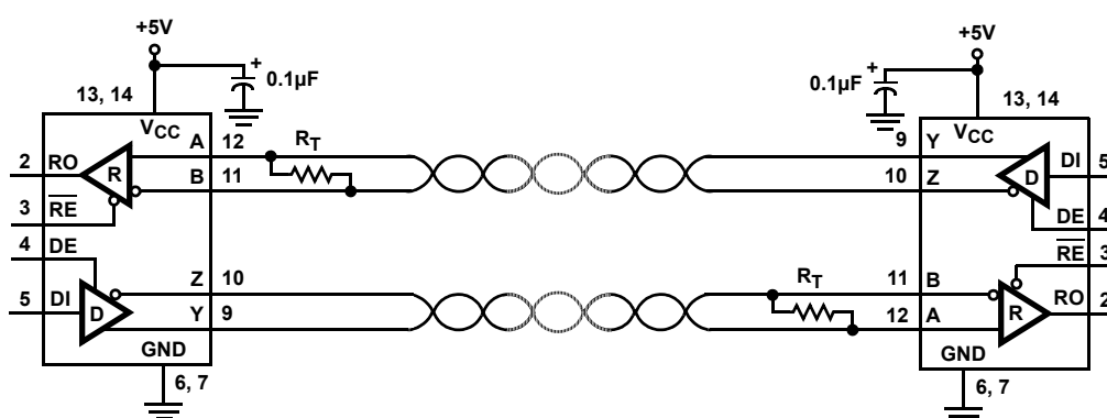
FIGURE 4. ISL31470E
