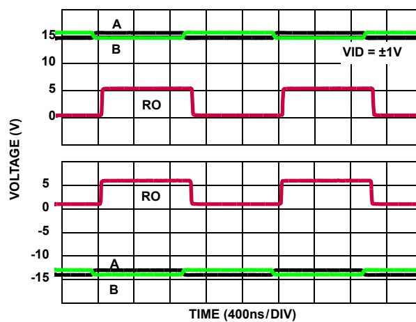
FIGURE 23. \pm 15V RECEIVER PERFORMANCE (ISL31475E)
