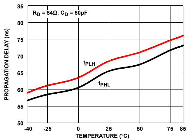
FIGURE 18. DRIVER DIFFERENTIAL PROPAGATION DELAY vs TEMPERATURE (ISL31475E)
