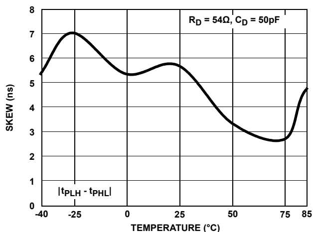
FIGURE 17. DRIVER DIFFERENTIAL SKEW vs TEMPERATURE (ISL31470E, ISL31472E)
